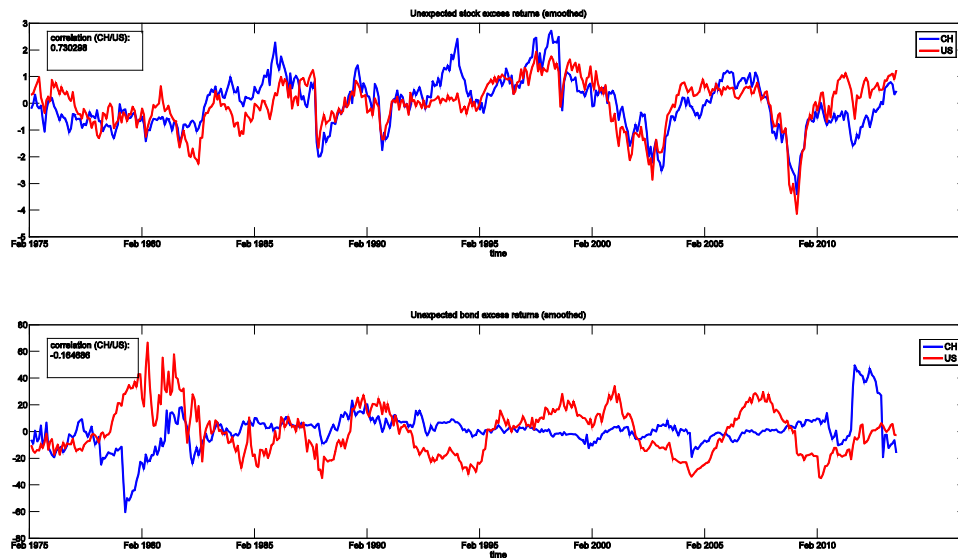
Figure 1: Time series of smoothed stock and bond excess return news.
